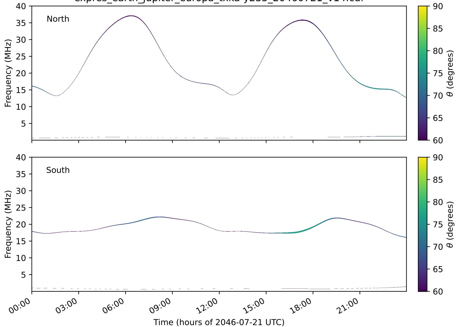
expres_earth_jupiter_europa_txka-y235_20460721_v14.cdf
