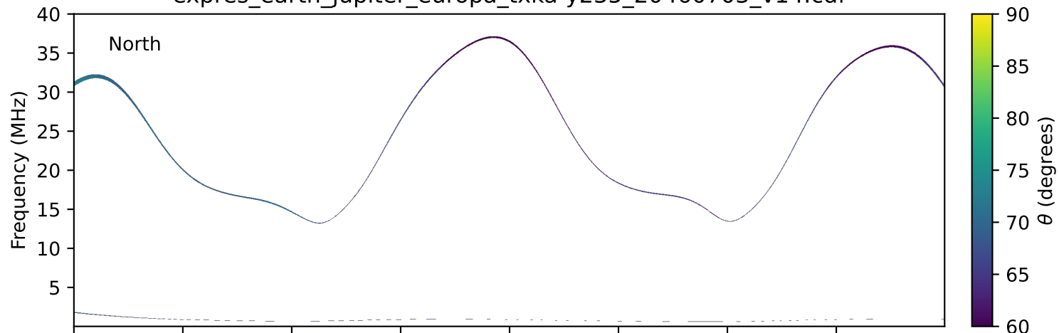
expres_earth_jupiter_europa_txka-y235_20460703_v14.cdf
