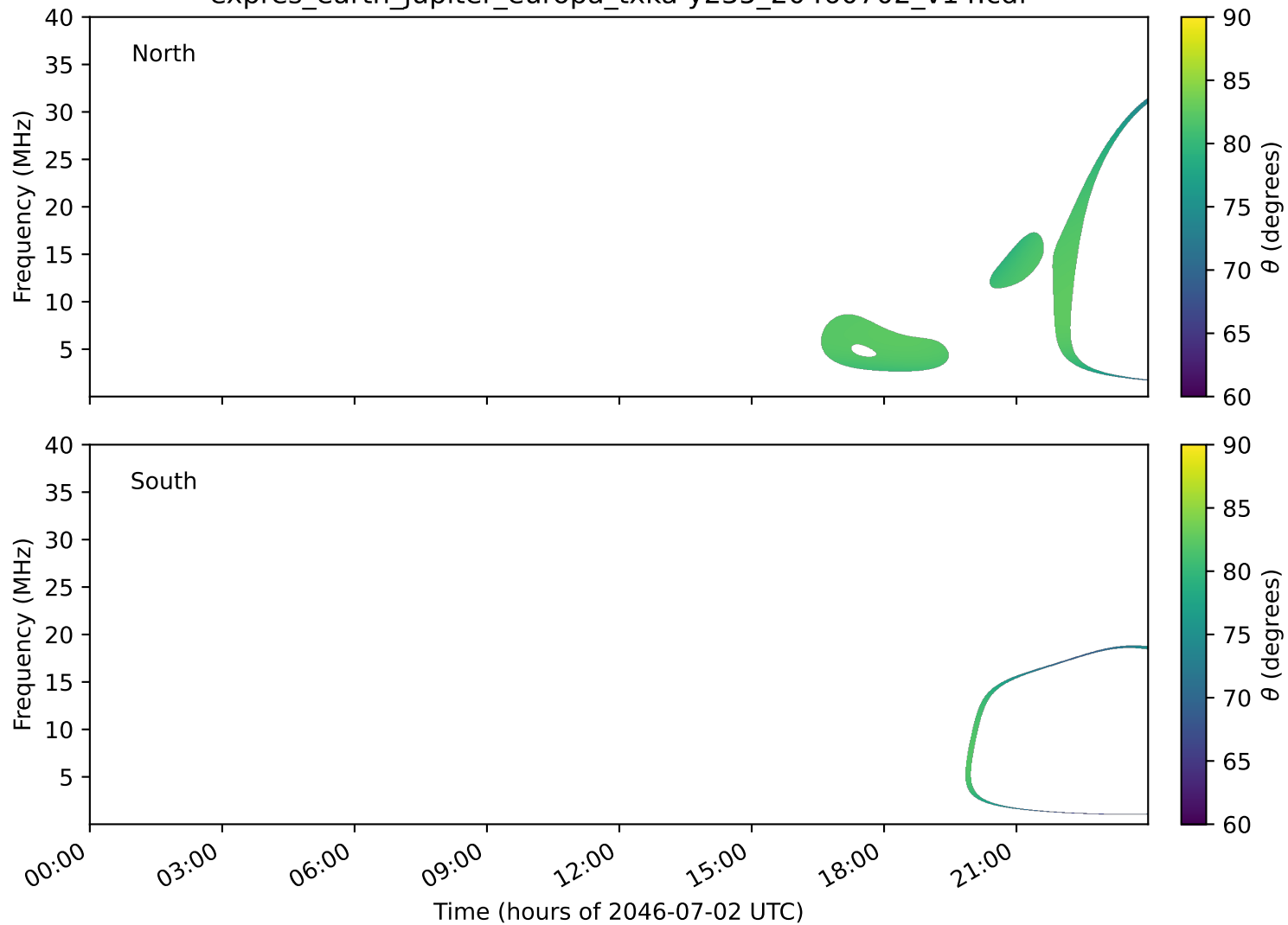
expres_earth_jupiter_europa_txka-y235_20460702_v14.cdf
