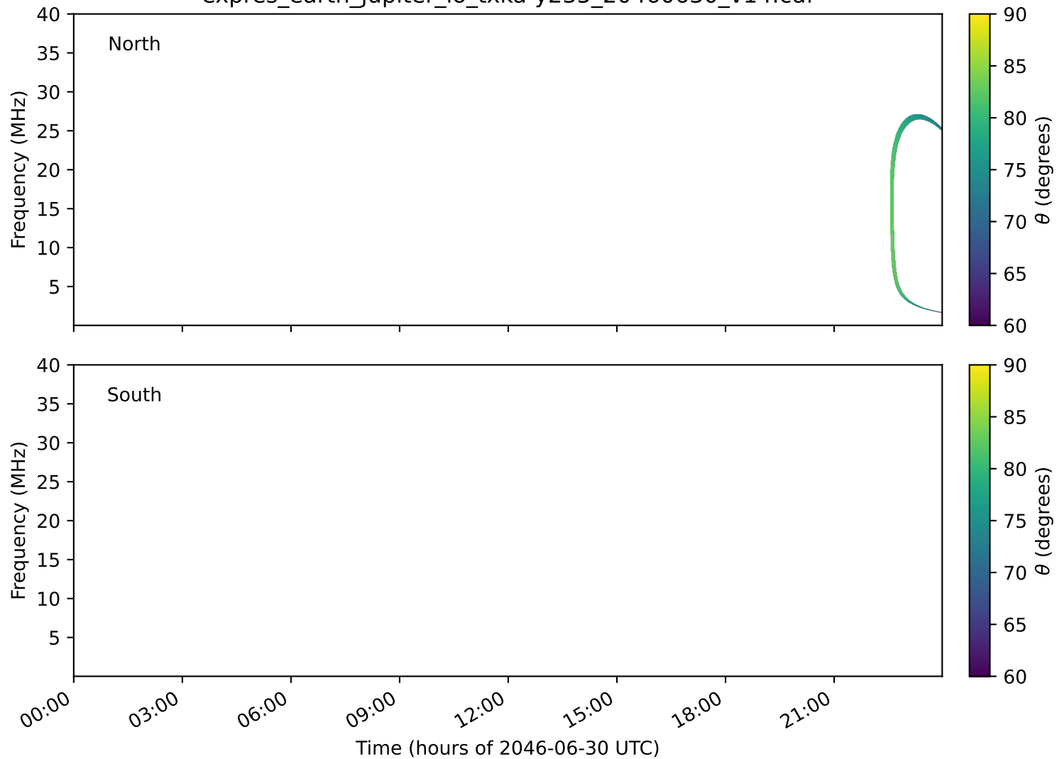
expres_earth_jupiter_io_txka-y235_20460630_v14.cdf
