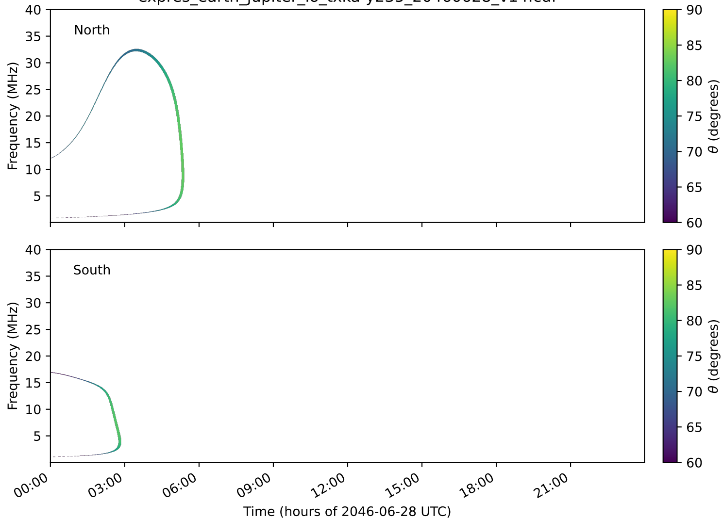
expres_earth_jupiter_io_txka-y235_20460628_v14.cdf
