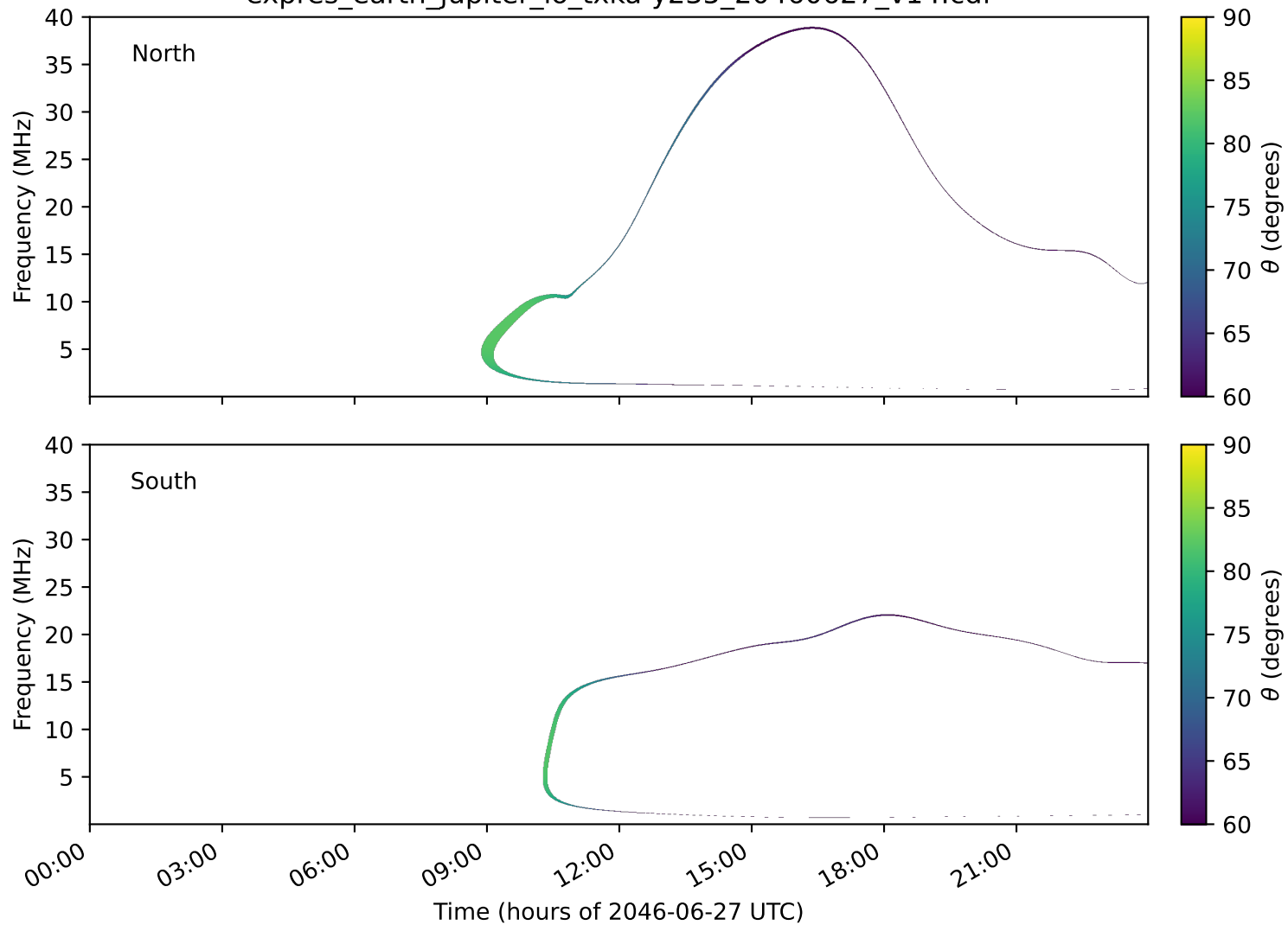
expres_earth_jupiter_io_txka-y235_20460627_v14.cdf
