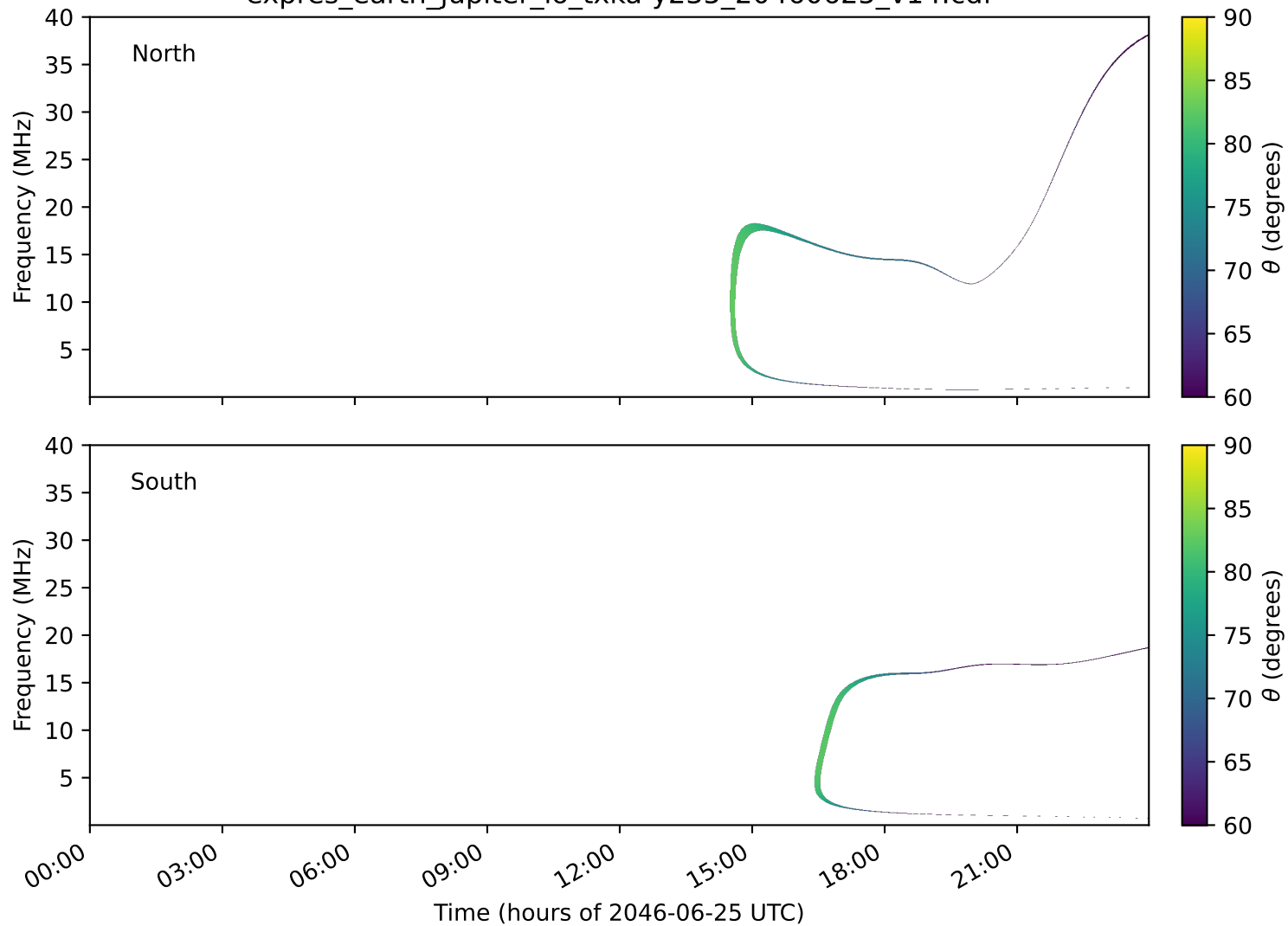
expres_earth_jupiter_io_txka-y235_20460625_v14.cdf
