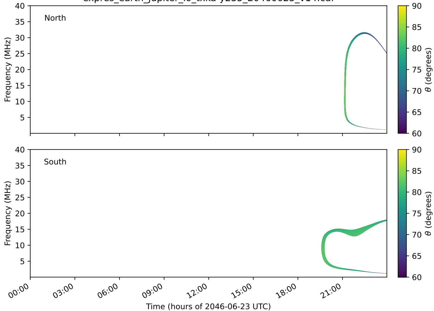
expres_earth_jupiter_io_txka-y235_20460623_v14.cdf
