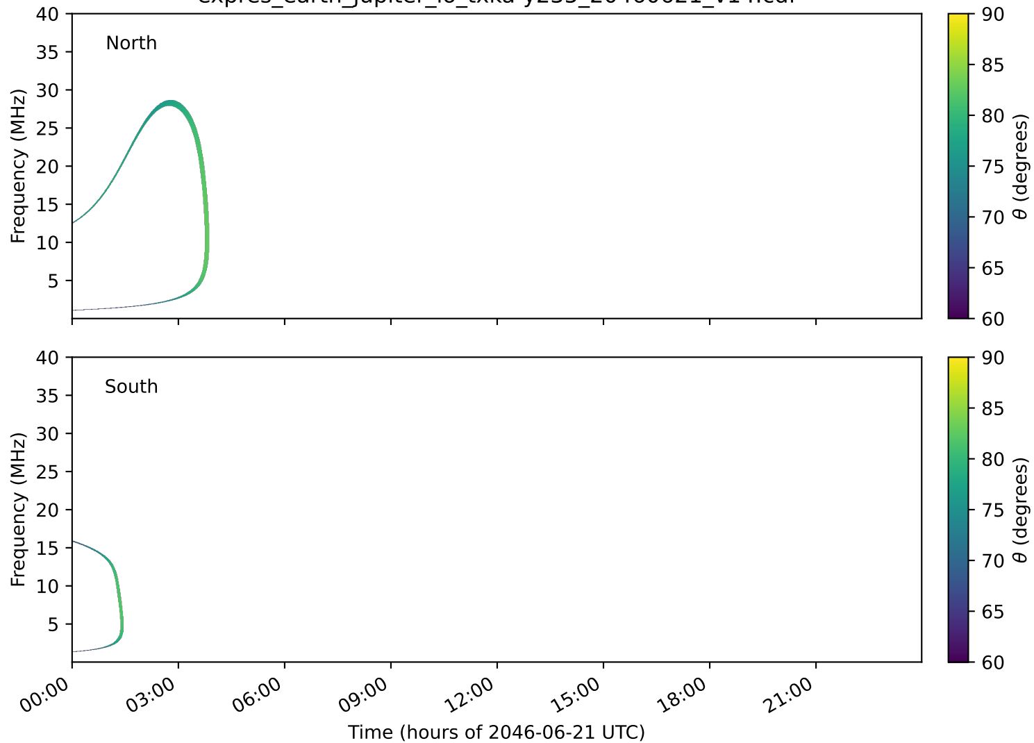
expres_earth_jupiter_io_txka-y235_20460621_v14.cdf
