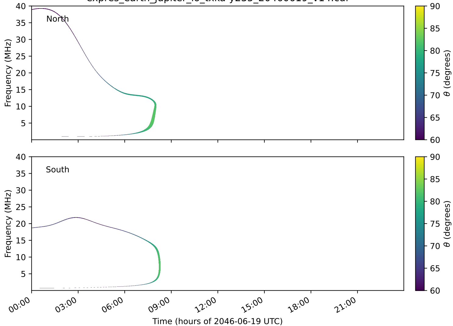
expres_earth_jupiter_io_txka-y235_20460619_v14.cdf
