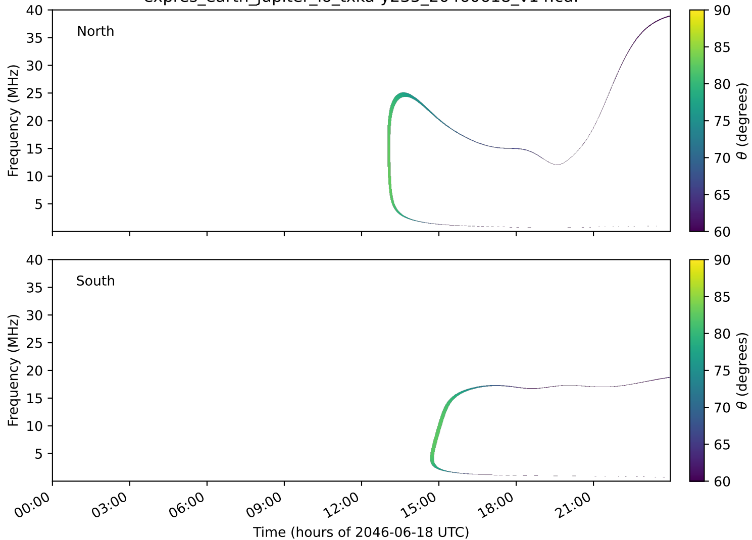
expres_earth_jupiter_io_txka-y235_20460618_v14.cdf
