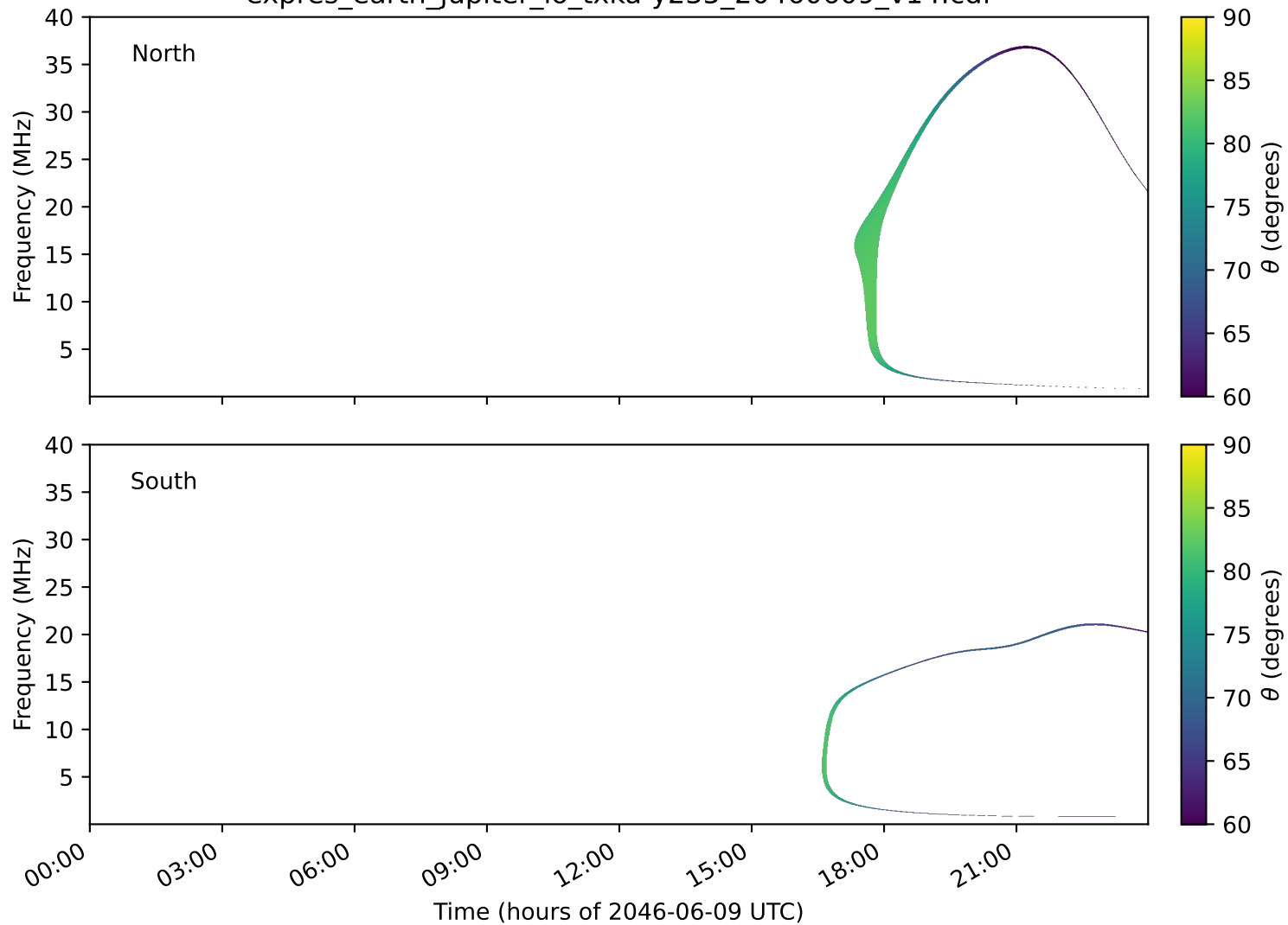
expres_earth_jupiter_io_txka-y235_20460609_v14.cdf
