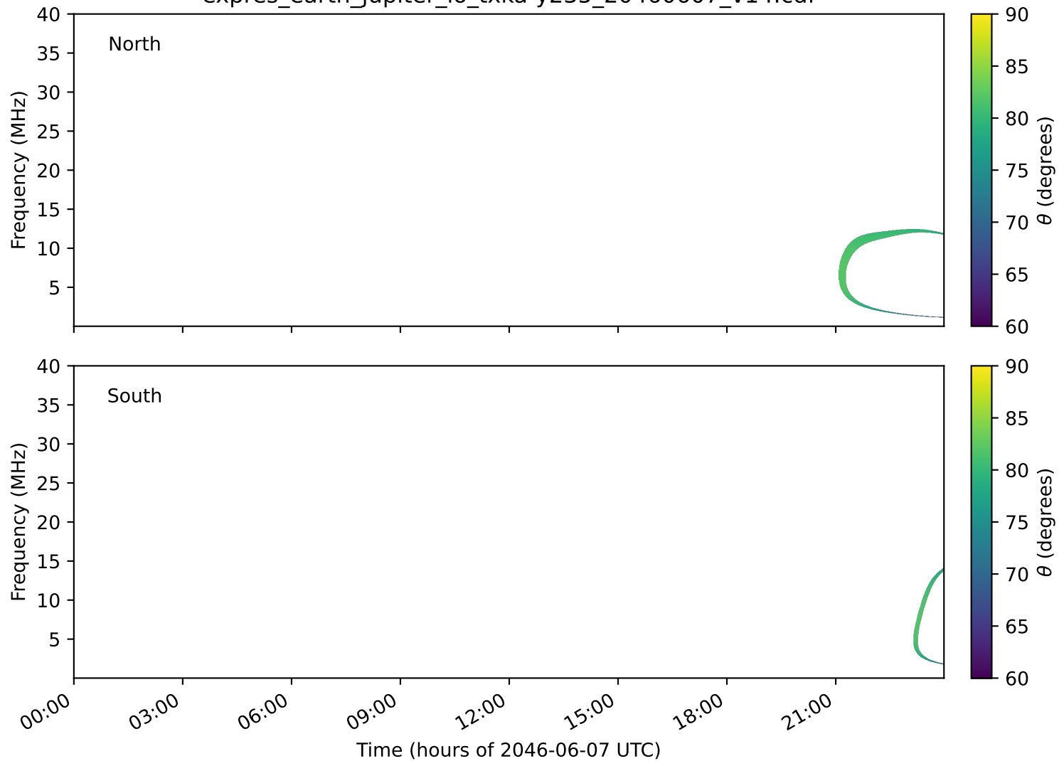
expres_earth_jupiter_io_txka-y235_20460607_v14.cdf
