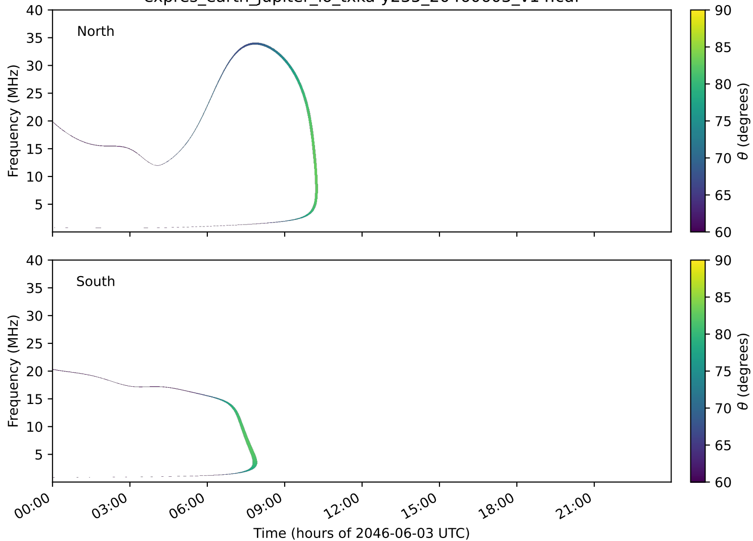
expres_earth_jupiter_io_txka-y235_20460603_v14.cdf
