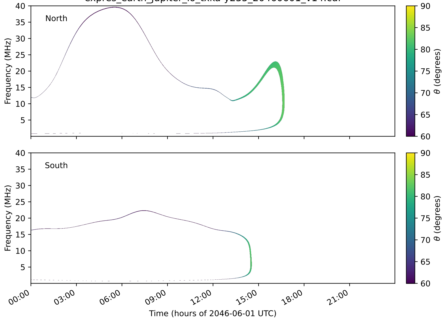
expres_earth_jupiter_io_txka-y235_20460601_v14.cdf
