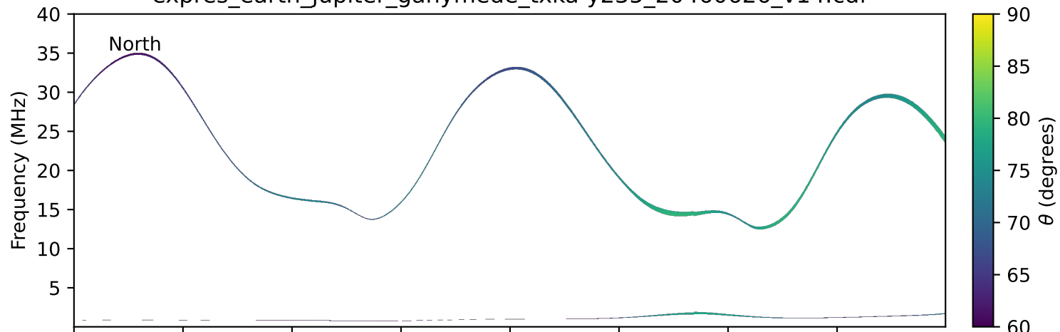
expres_earth_jupiter_ganymede_txka-y235_20460626_v14.cdf
