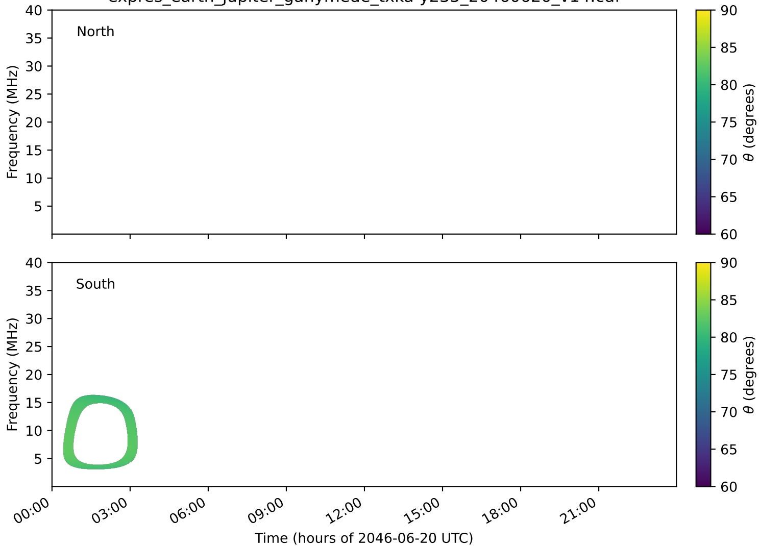
expres_earth_jupiter_ganymede_txka-y235_20460620_v14.cdf
