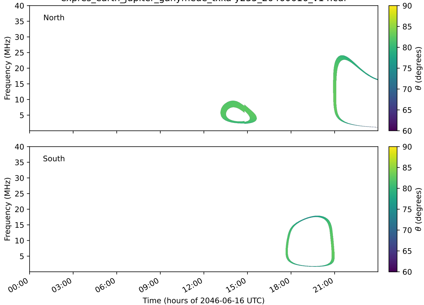
expres_earth_jupiter_ganymede_txka-y235_20460616_v14.cdf
