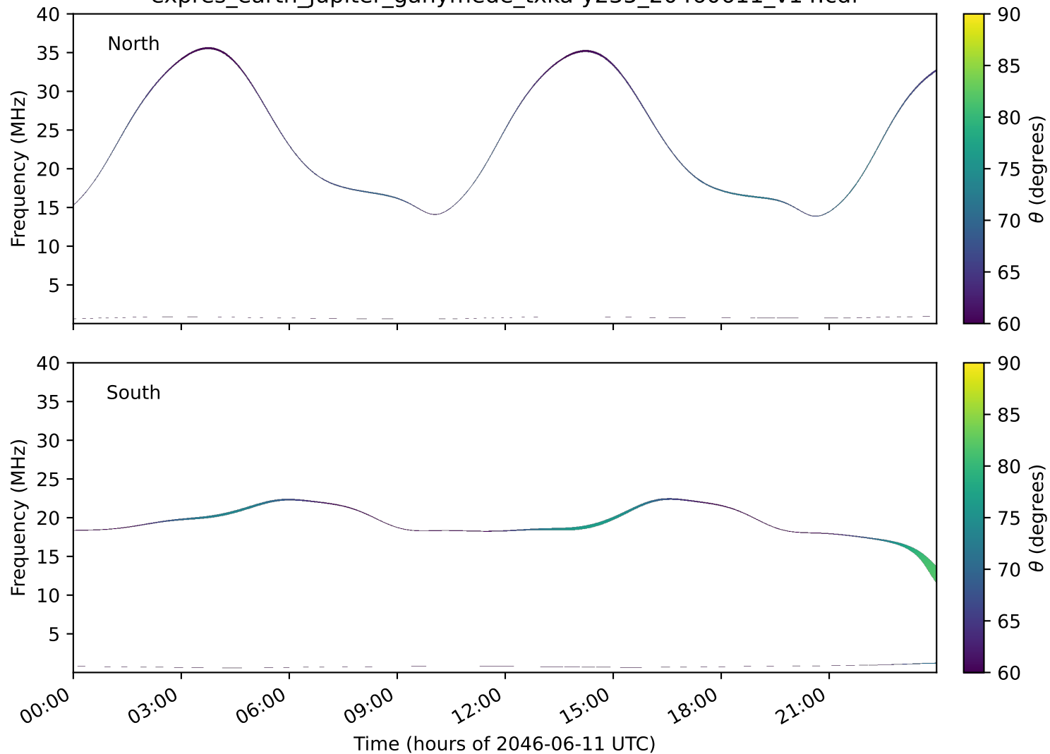
expres_earth_jupiter_ganymede_txka-y235_20460611_v14.cdf
