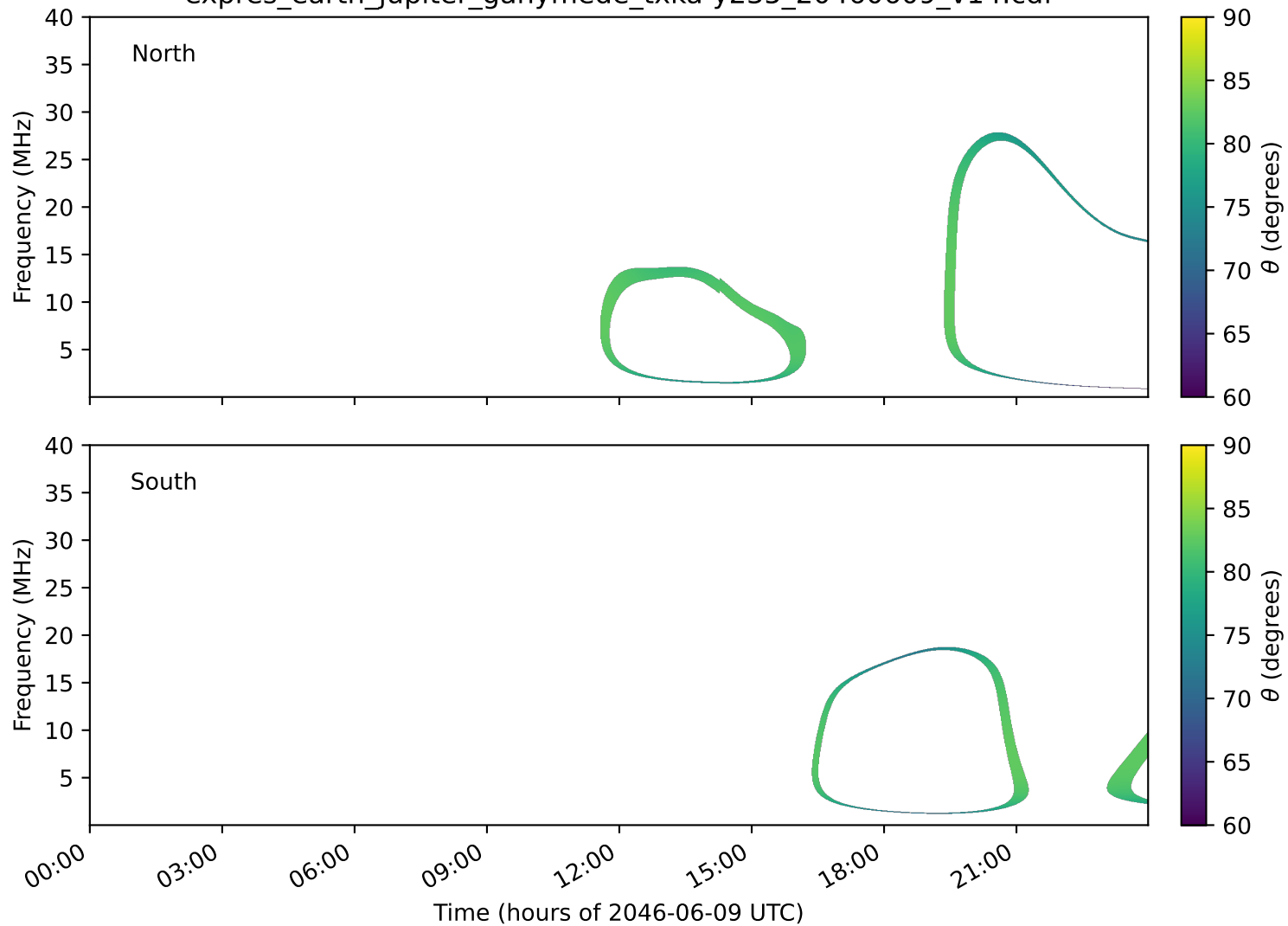
expres_earth_jupiter_ganymede_txka-y235_20460609_v14.cdf
