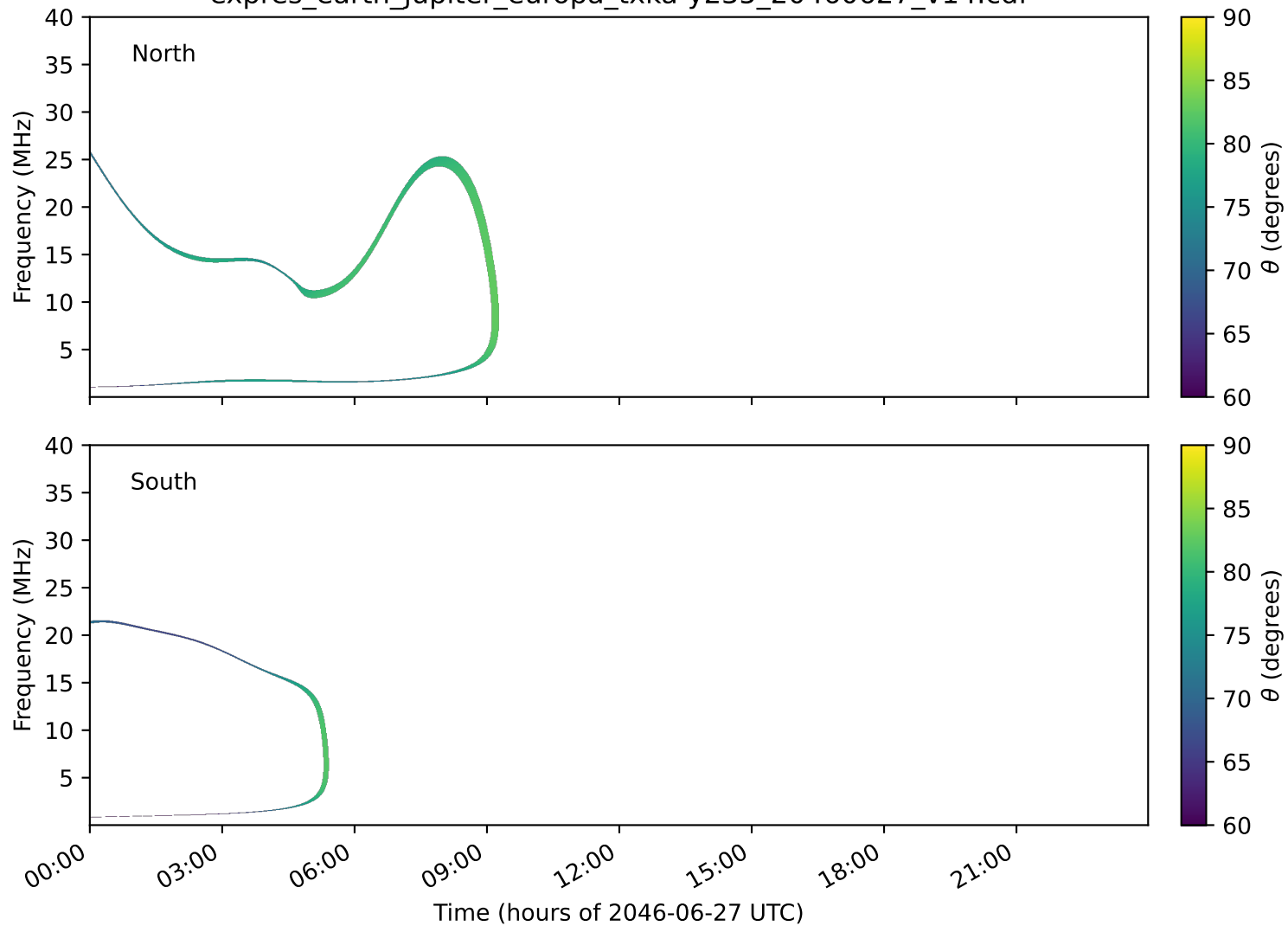
expres_earth_jupiter_europa_txka-y235_20460627_v14.cdf
