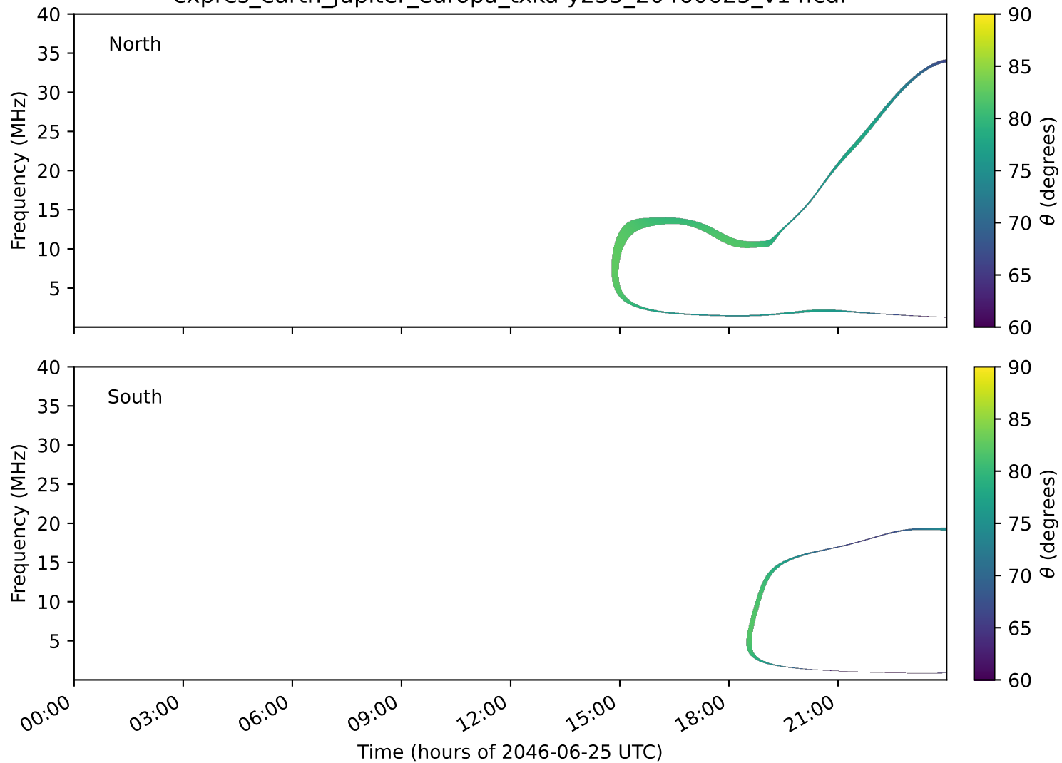
expres_earth_jupiter_europa_txka-y235_20460625_v14.cdf
