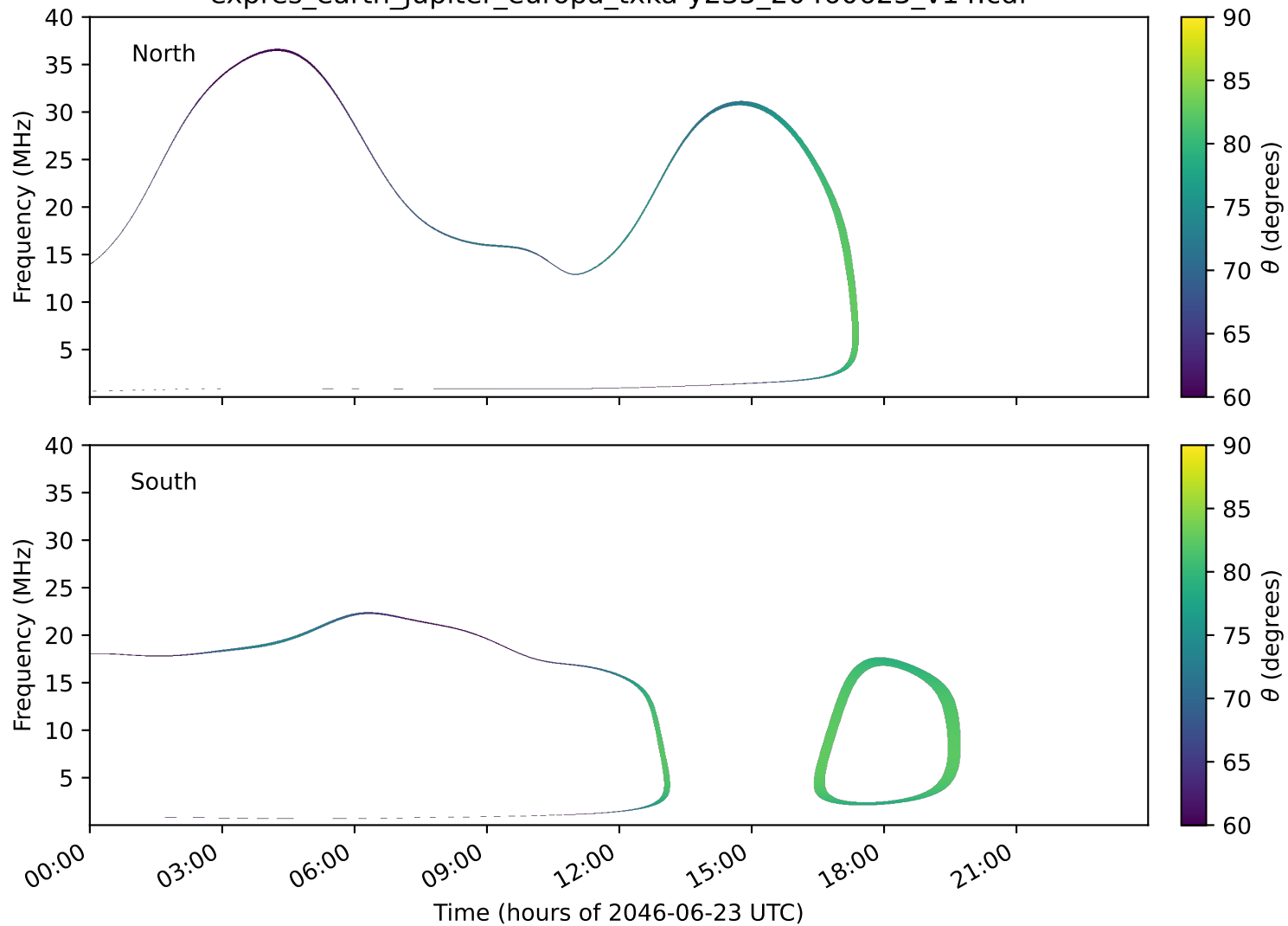
expres_earth_jupiter_europa_txka-y235_20460623_v14.cdf
