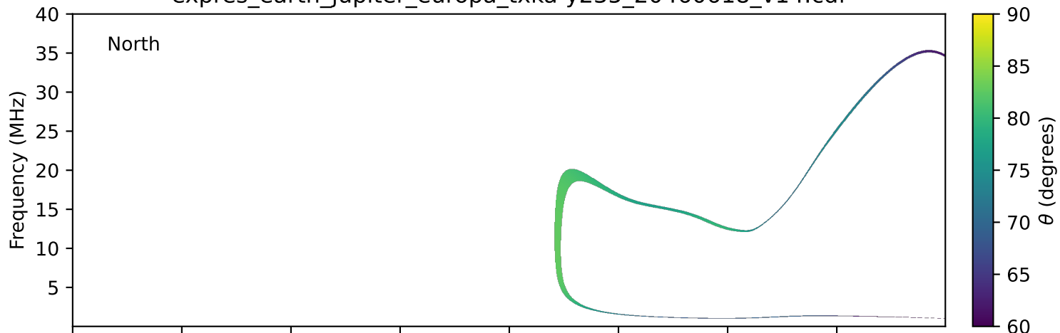
expres_earth_jupiter_europa_txka-y235_20460618_v14.cdf
