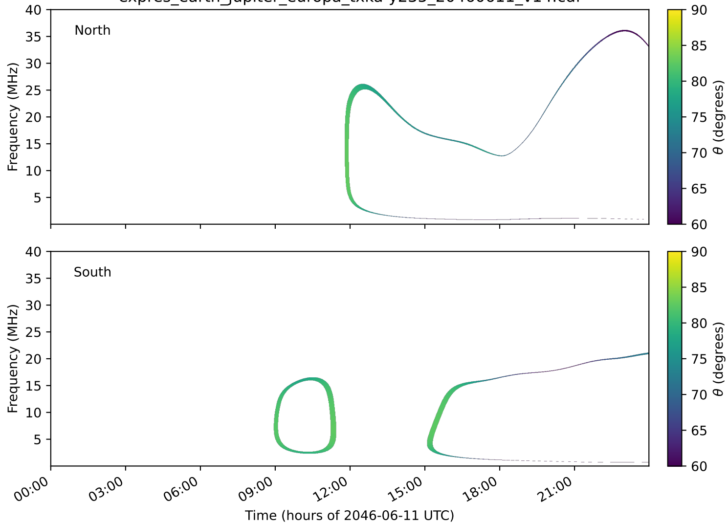
expres_earth_jupiter_europa_txka-y235_20460611_v14.cdf
