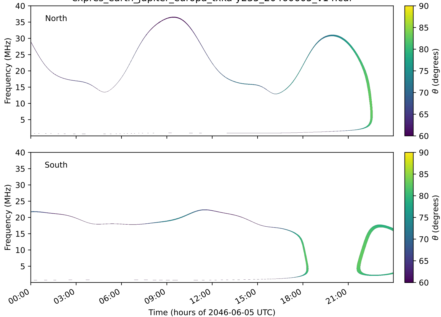
expres_earth_jupiter_europa_txka-y235_20460605_v14.cdf
