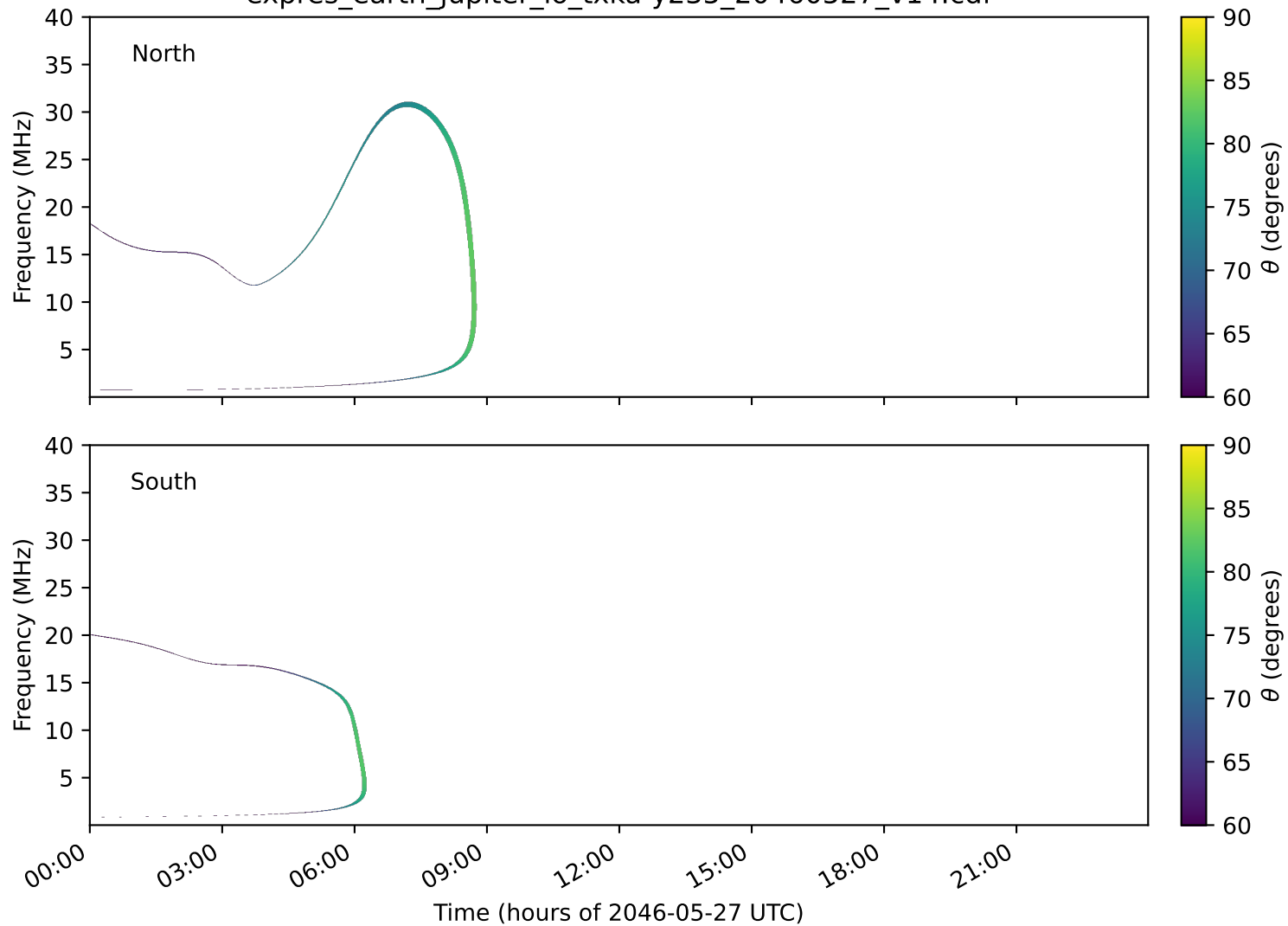
expres_earth_jupiter_io_txka-y235_20460527_v14.cdf
