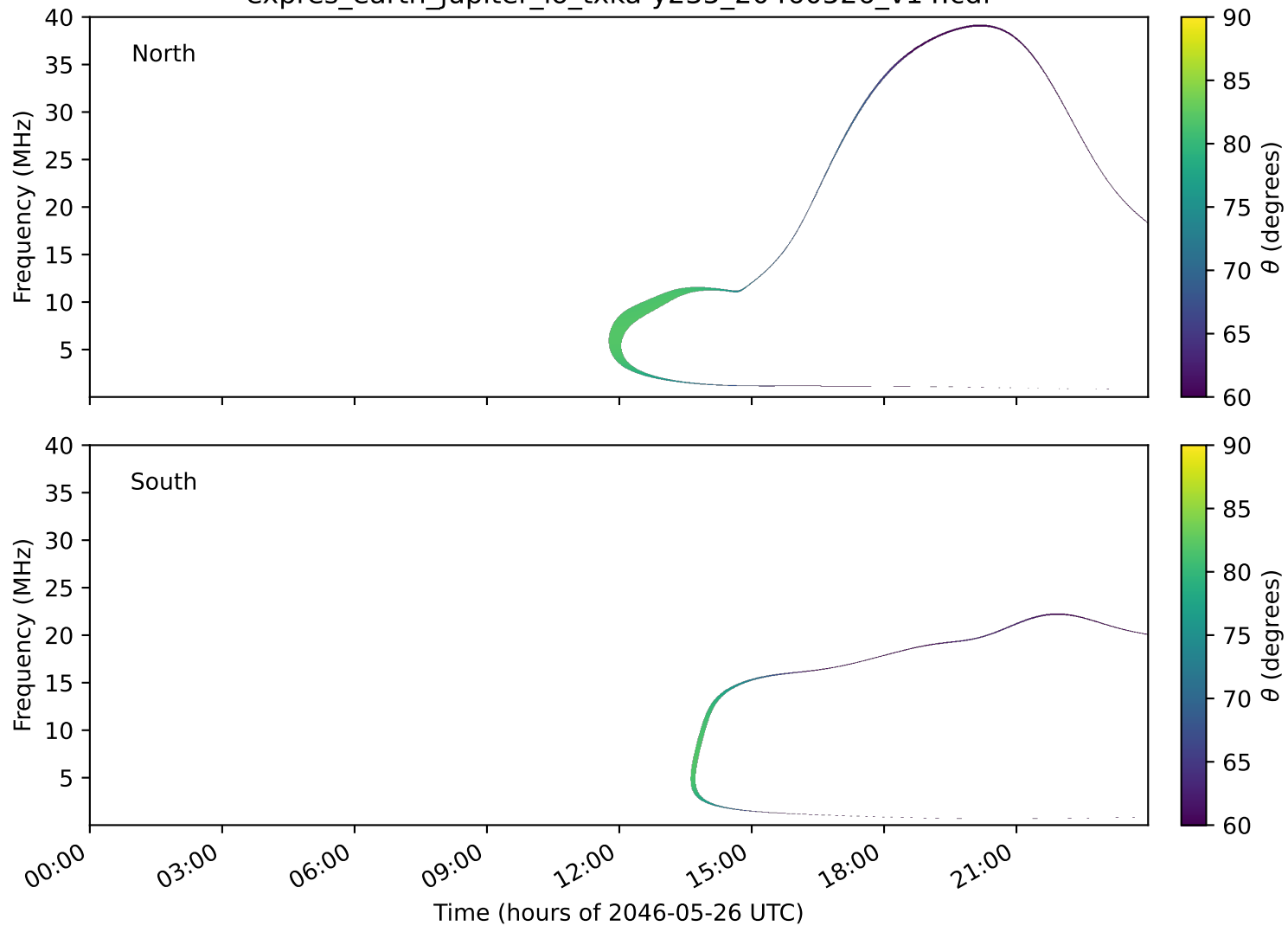
expres_earth_jupiter_io_txka-y235_20460526_v14.cdf
