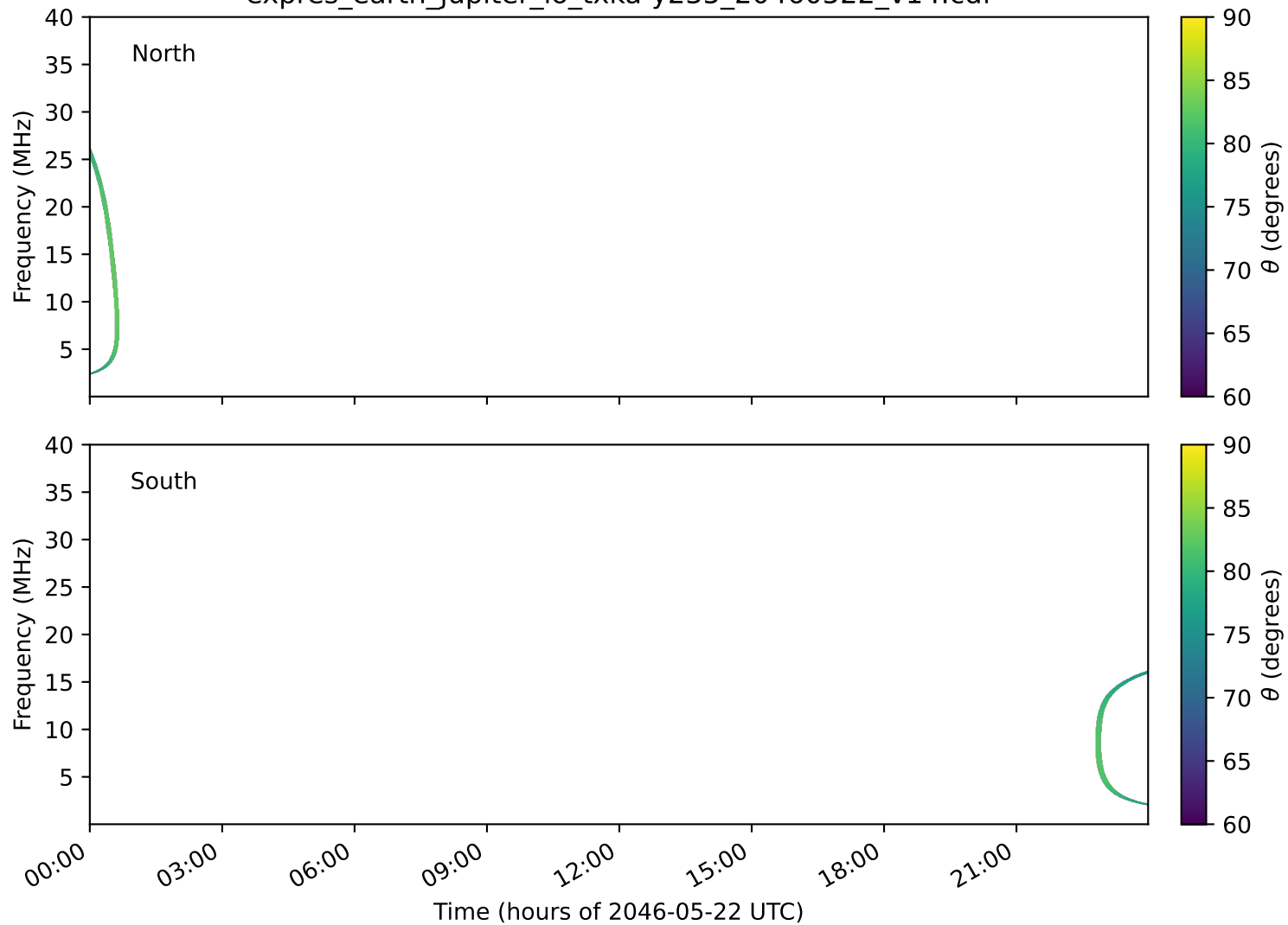
expres_earth_jupiter_io_txka-y235_20460522_v14.cdf
