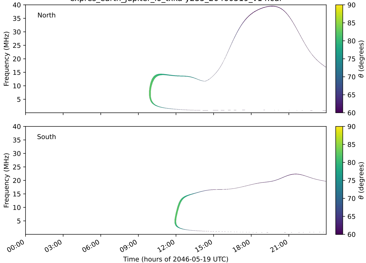
expres_earth_jupiter_io_txka-y235_20460519_v14.cdf
