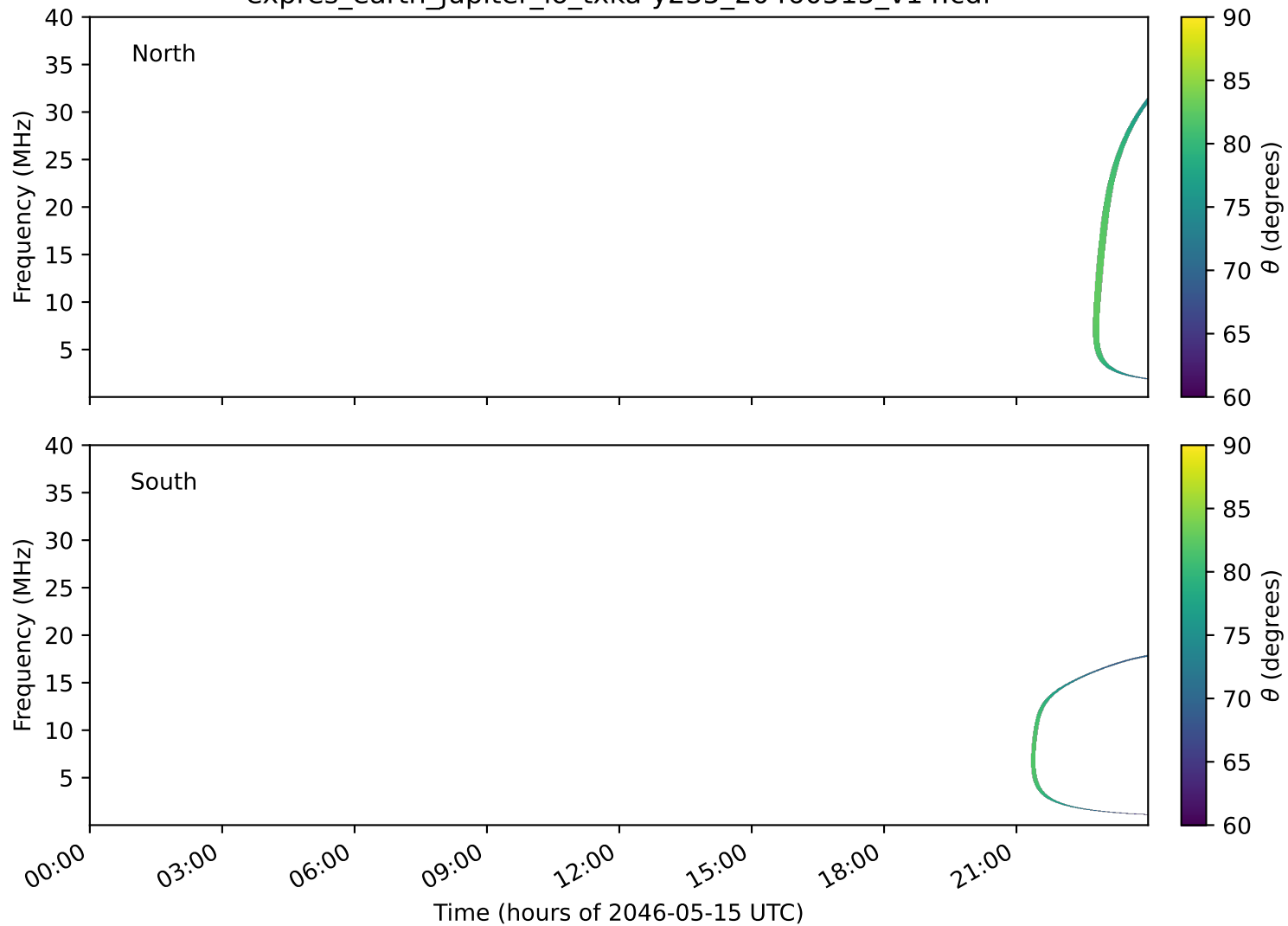
expres_earth_jupiter_io_txka-y235_20460515_v14.cdf
