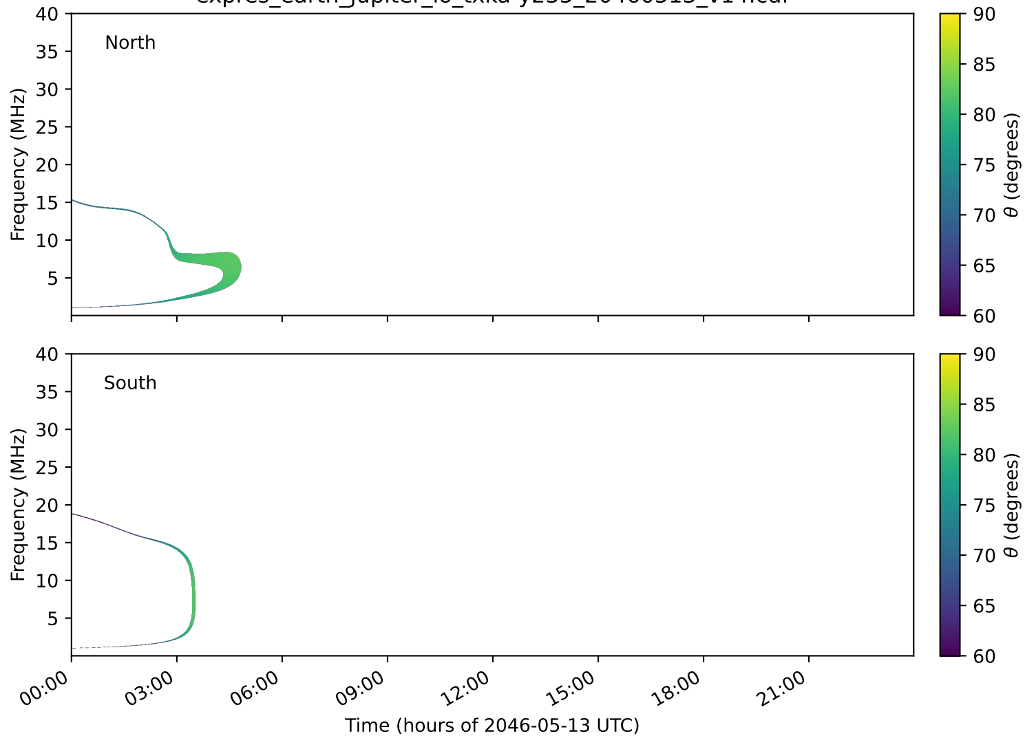
expres_earth_jupiter_io_txka-y235_20460513_v14.cdf
