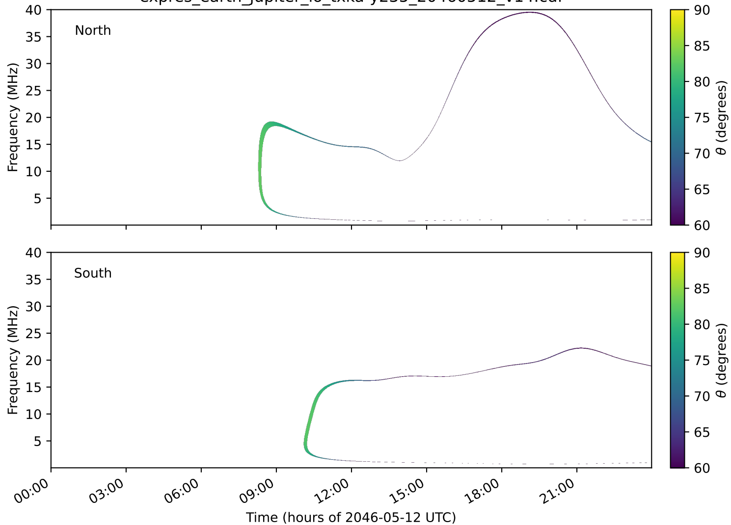
expres_earth_jupiter_io_txka-y235_20460512_v14.cdf
