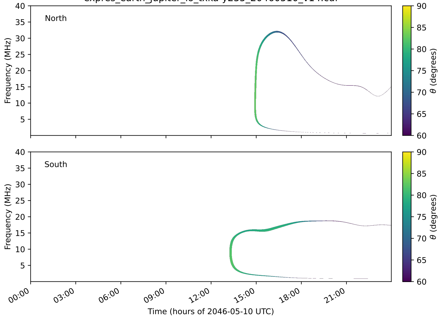
expres_earth_jupiter_io_txka-y235_20460510_v14.cdf
