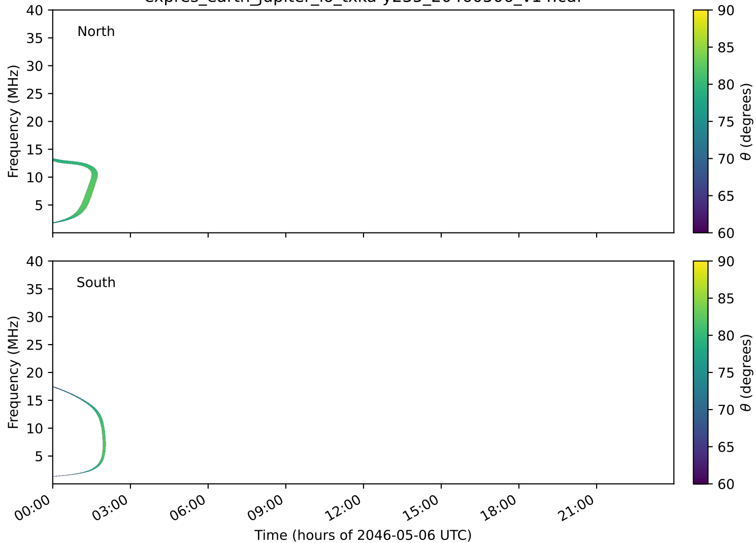
expres_earth_jupiter_io_txka-y235_20460506_v14.cdf
