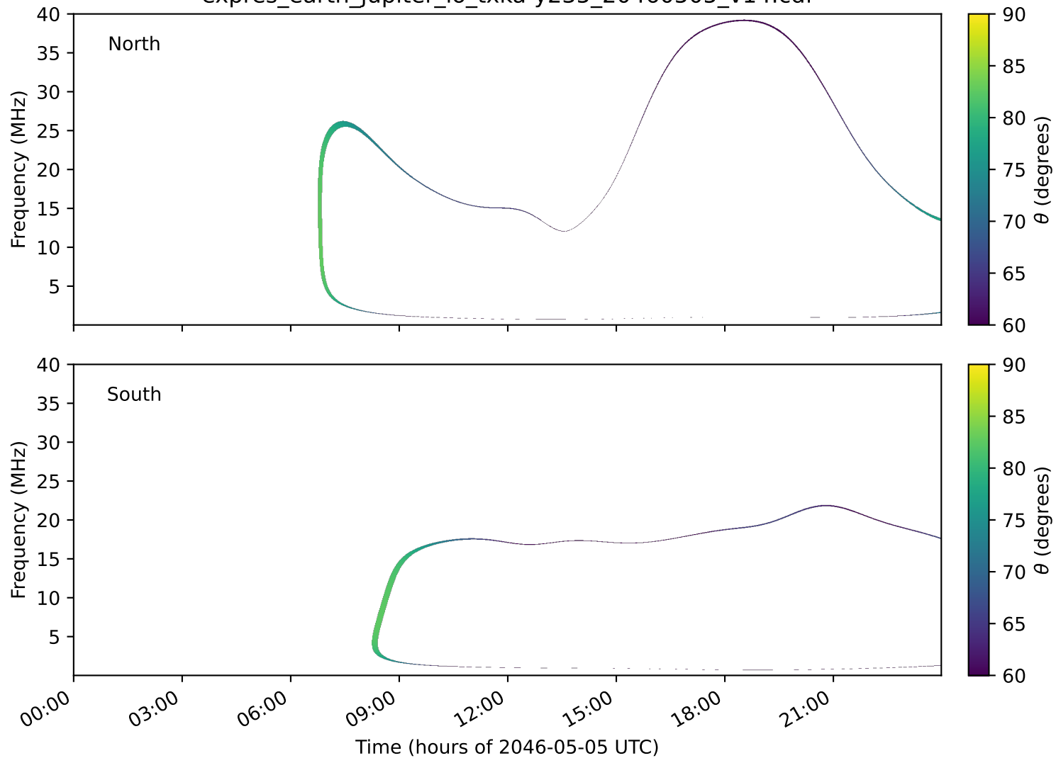
expres_earth_jupiter_io_txka-y235_20460505_v14.cdf
