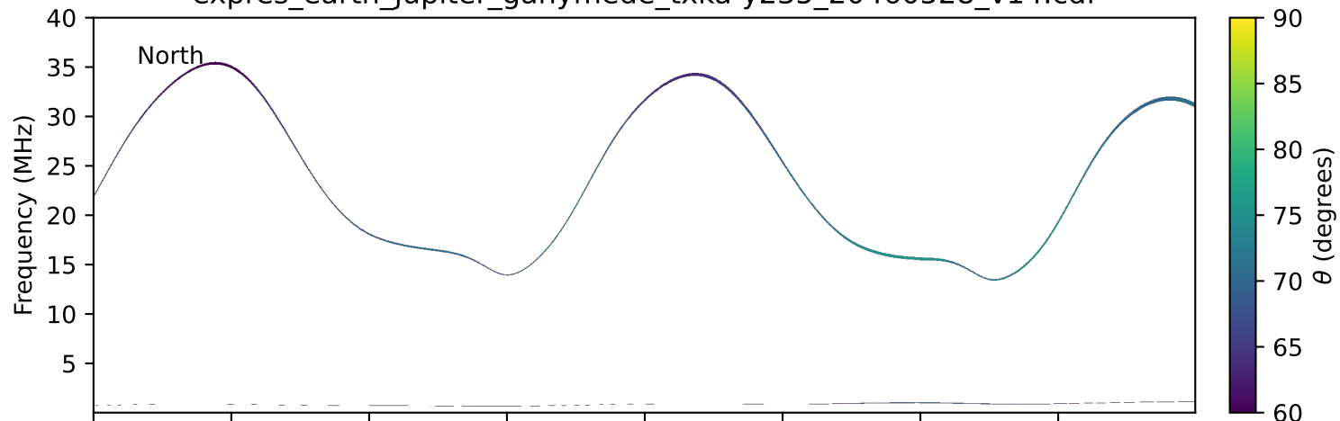
expres_earth_jupiter_ganymede_txka-y235_20460528_v14.cdf
