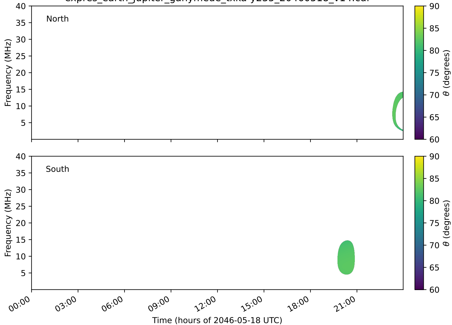
expres_earth_jupiter_ganymede_txka-y235_20460518_v14.cdf
