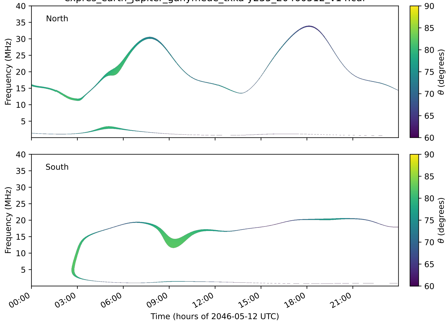
expres_earth_jupiter_ganymede_txka-y235_20460512_v14.cdf
