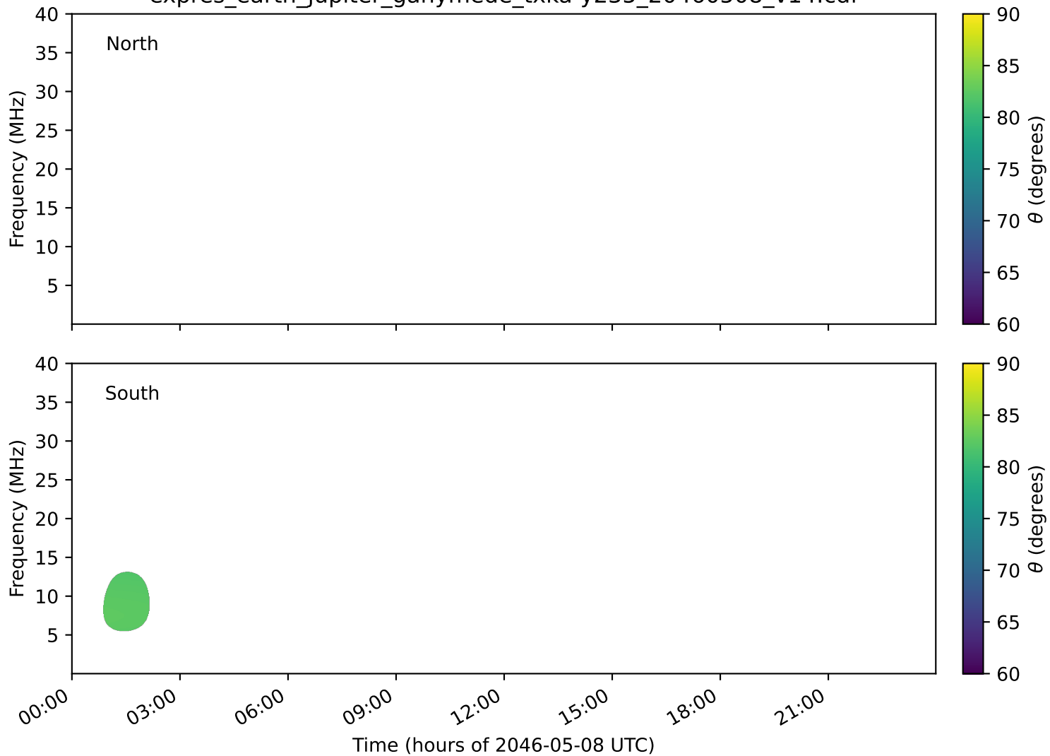
expres_earth_jupiter_ganymede_txka-y235_20460508_v14.cdf
