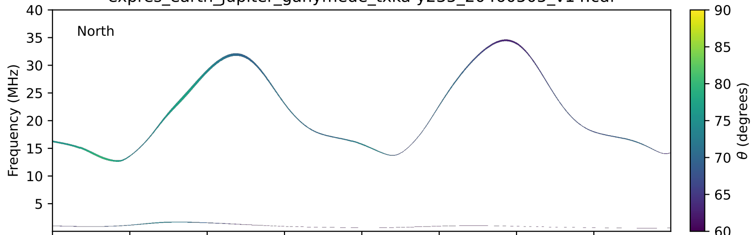
expres_earth_jupiter_ganymede_txka-y235_20460505_v14.cdf
