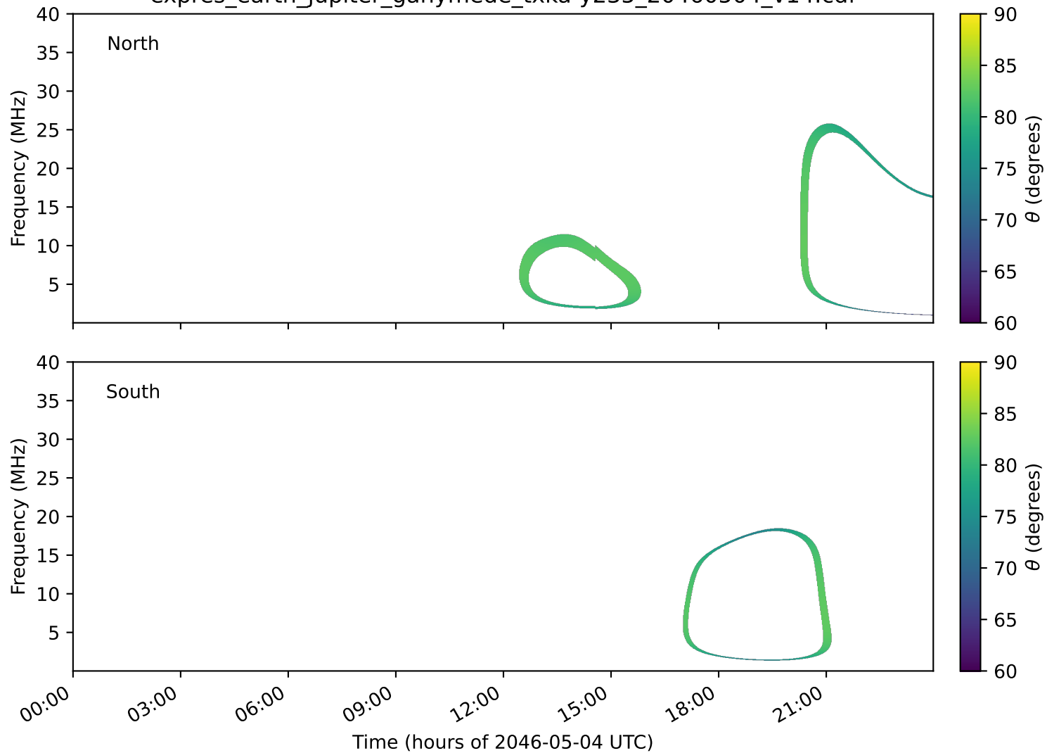
expres_earth_jupiter_ganymede_txka-y235_20460504_v14.cdf
