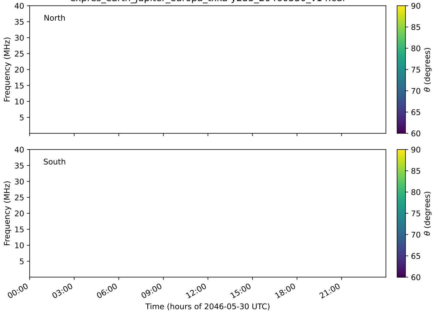
expres_earth_jupiter_europa_txka-y235_20460530_v14.cdf
