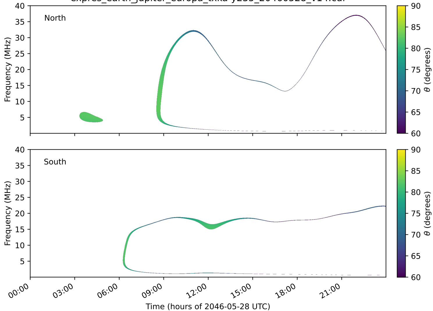
expres_earth_jupiter_europa_txka-y235_20460528_v14.cdf
