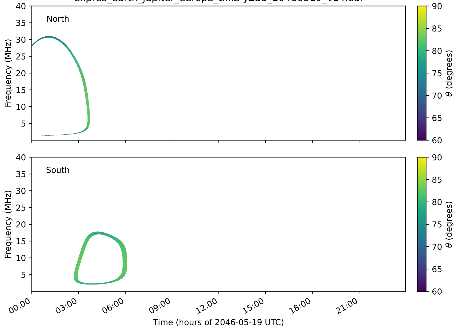
expres_earth_jupiter_europa_txka-y235_20460519_v14.cdf
