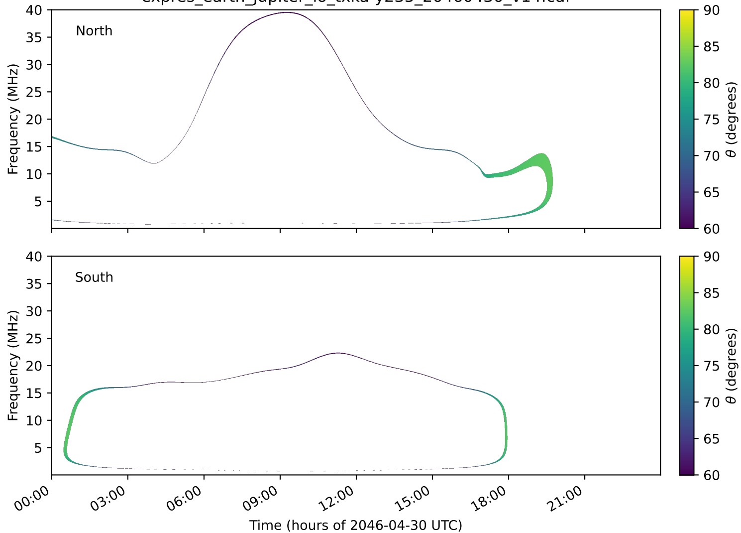
expres_earth_jupiter_io_txka-y235_20460430_v14.cdf
