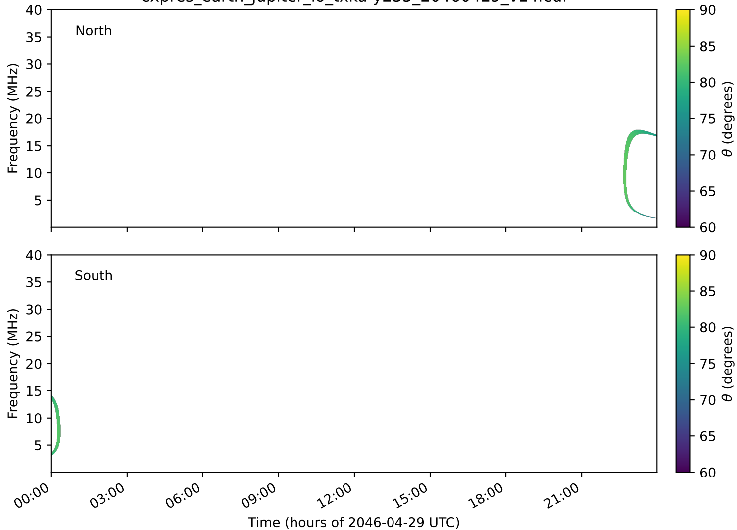
expres_earth_jupiter_io_txka-y235_20460429_v14.cdf
