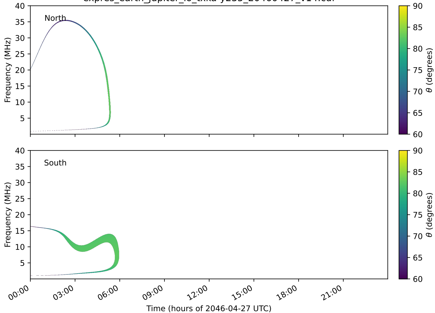
expres_earth_jupiter_io_txka-y235_20460427_v14.cdf
