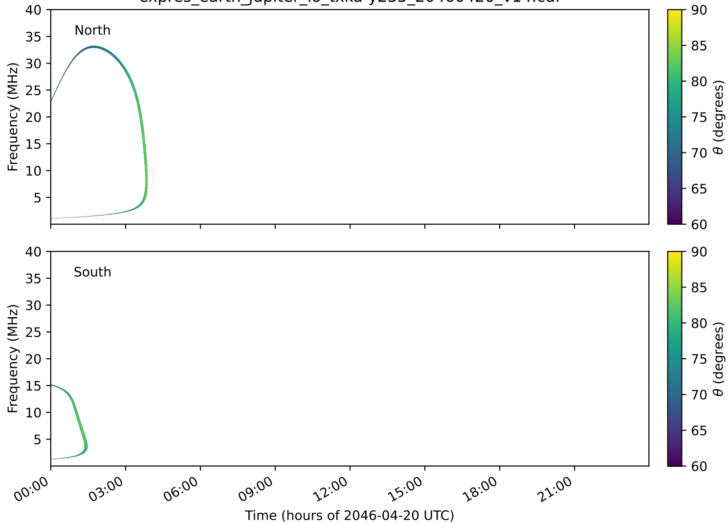
expres_earth_jupiter_io_txka-y235_20460420_v14.cdf
