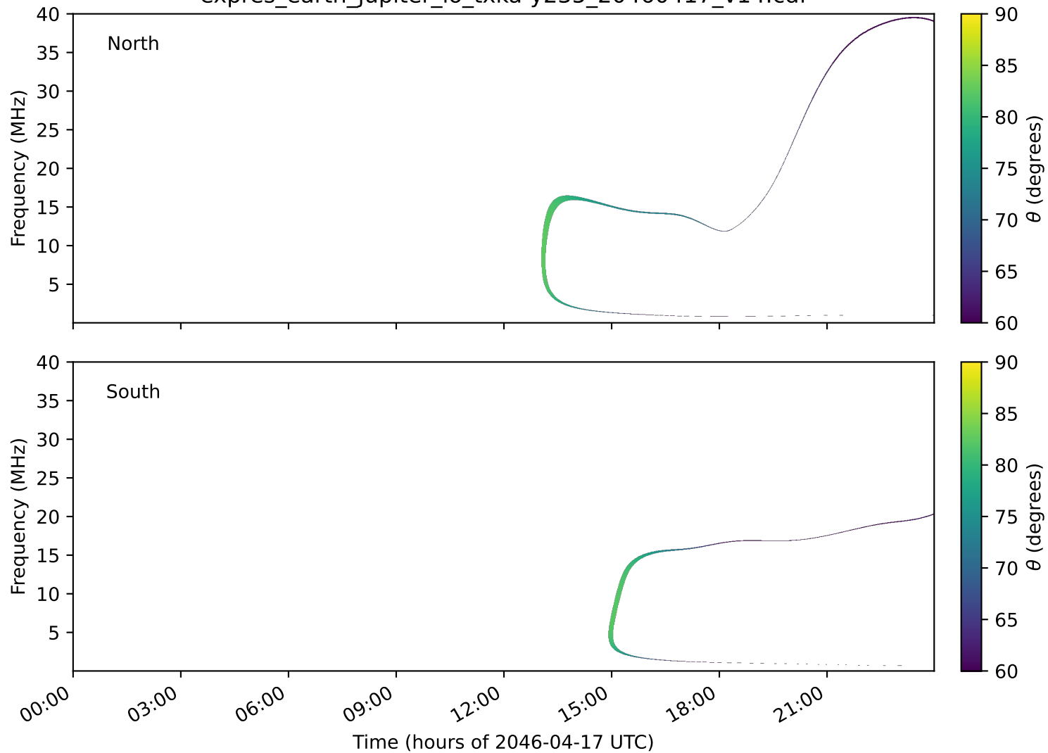
expres_earth_jupiter_io_txka-y235_20460417_v14.cdf
